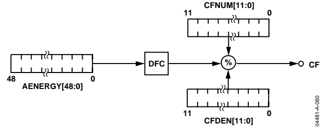
Figure 59. Energy-to-Frequency Conversion
