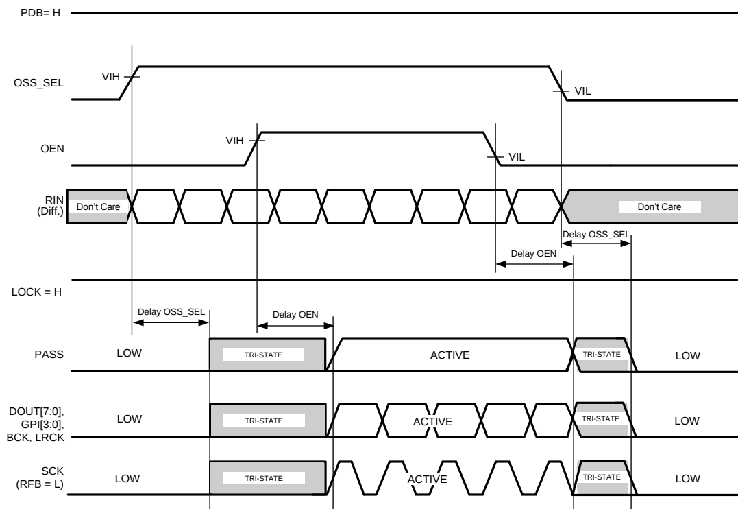
Figure 11. Output States
