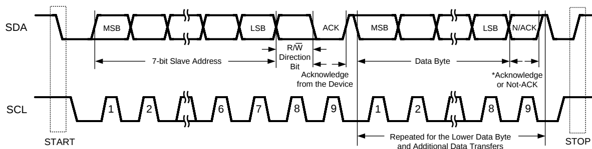
Figure 20. Basic Operation
