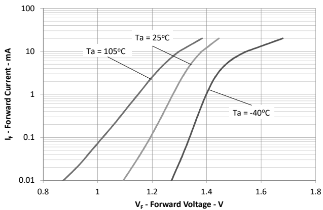
Figure 7: Typical Input Diode Forward Characteristics
