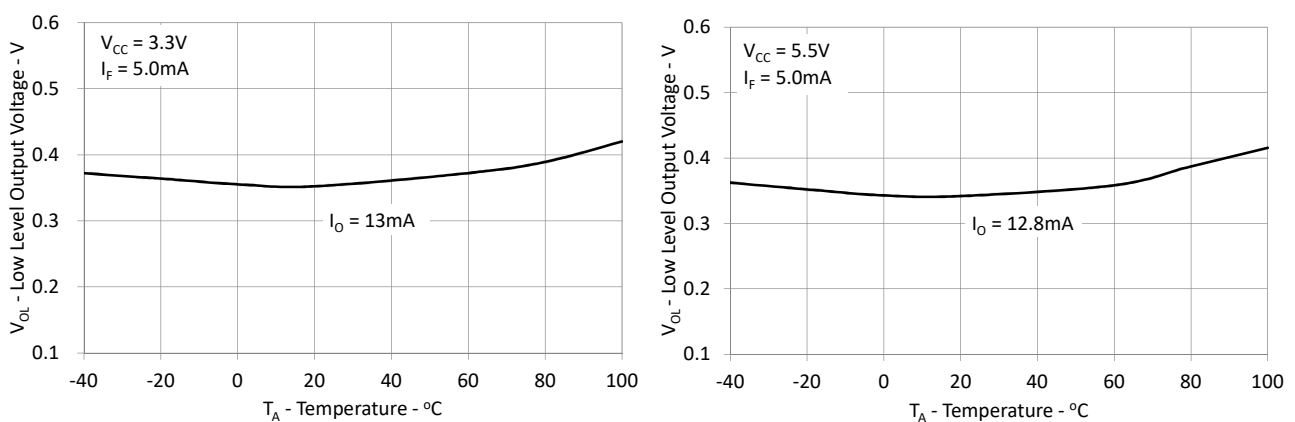
Figure 5: Typical Low Level Output Voltage vs. Ambient Temperature
