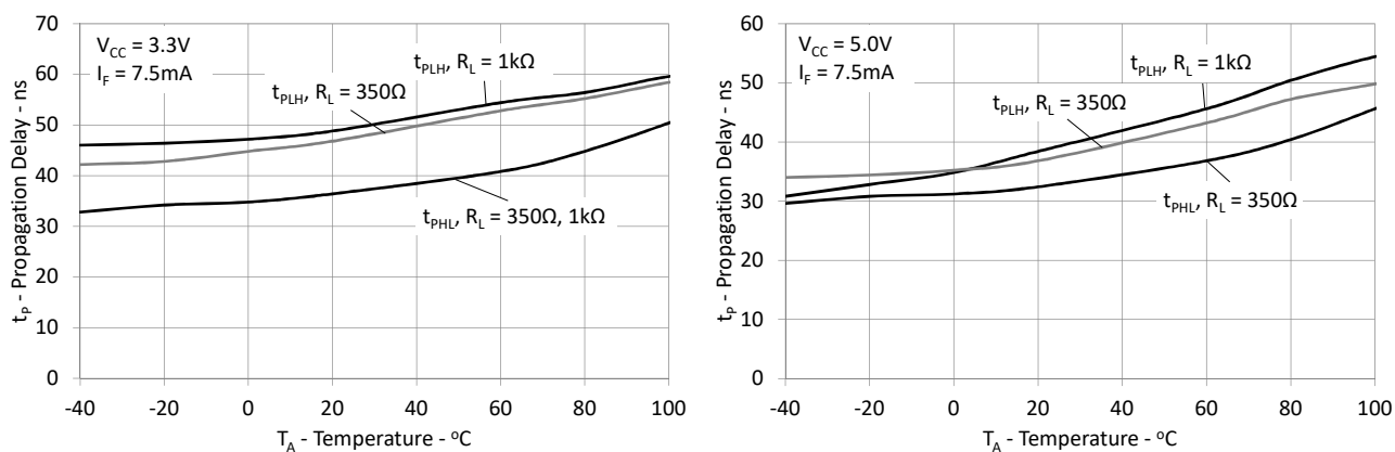
Figure 8: Typical Propagation Delay vs. Ambient Temperature
