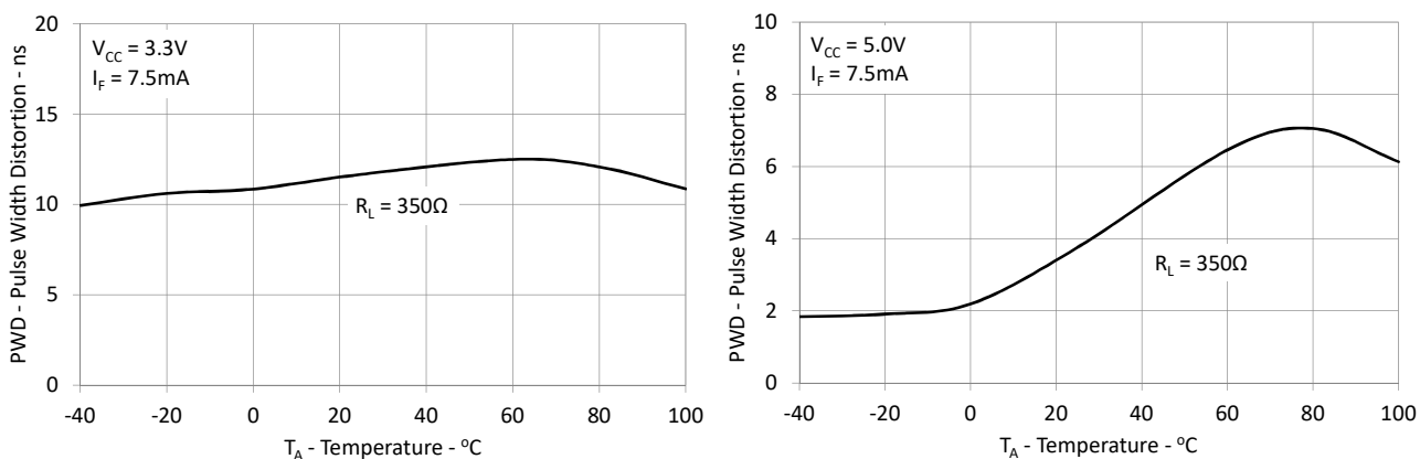
Figure 9: Typical Pulse Width Distortion vs. Ambient Temperature
