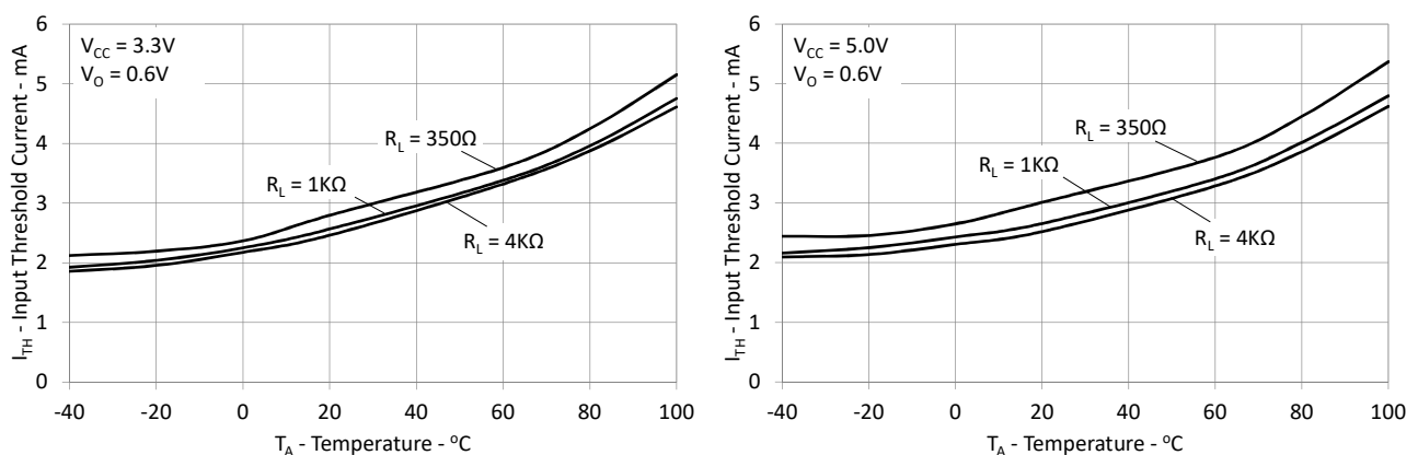
Figure 4: Typical Input Diode Threshold Current vs. Ambient Temperature
