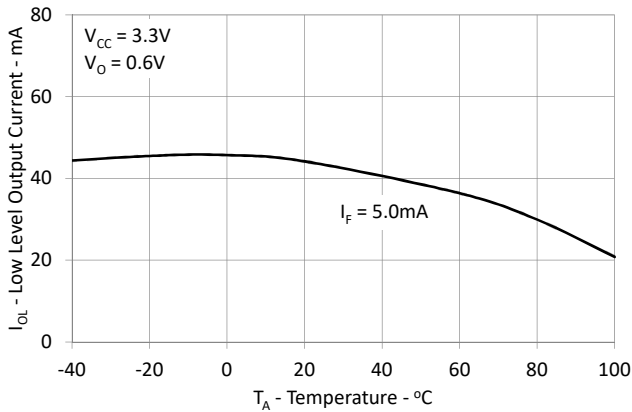
Figure 6: Typical Low Level Output Current vs. Ambient Temperature
