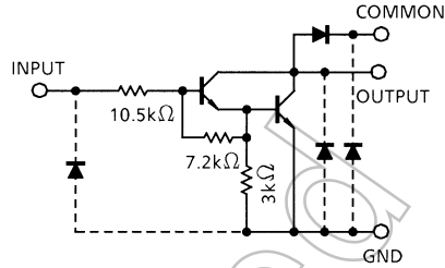
TD62004APG/AFG
