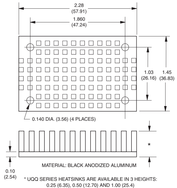
Figure 8. Optional Heatsink
