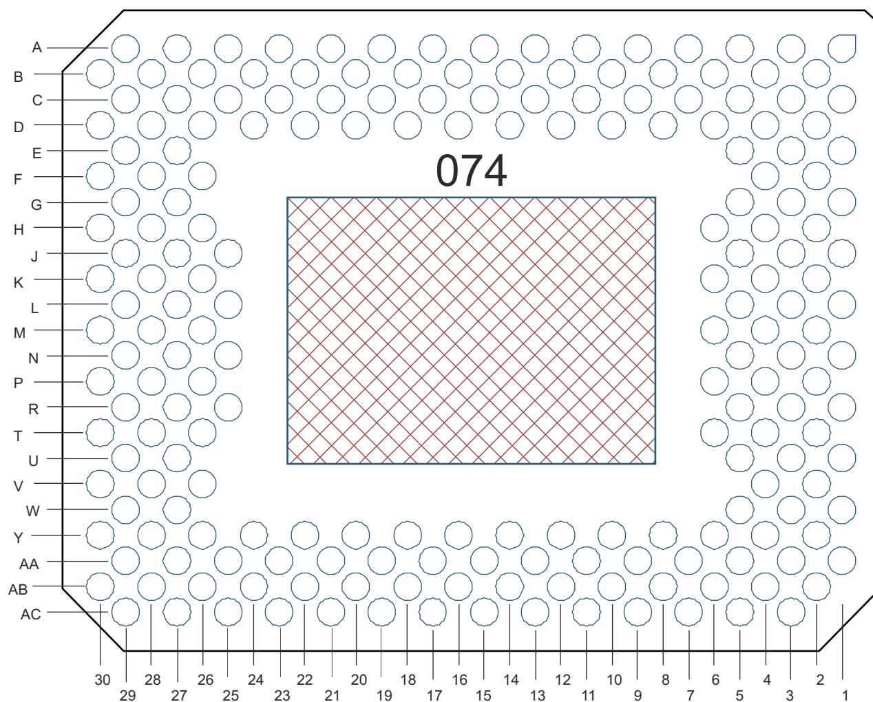
Figure 6-1. FLP Package 203-Pin CLGA Bottom View
