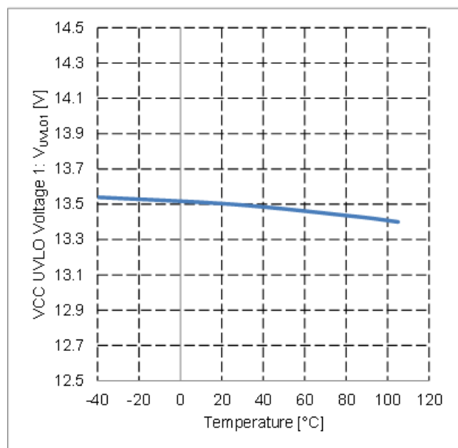
Figure 18. VCC UVLO Voltage 1 vs Temperature
