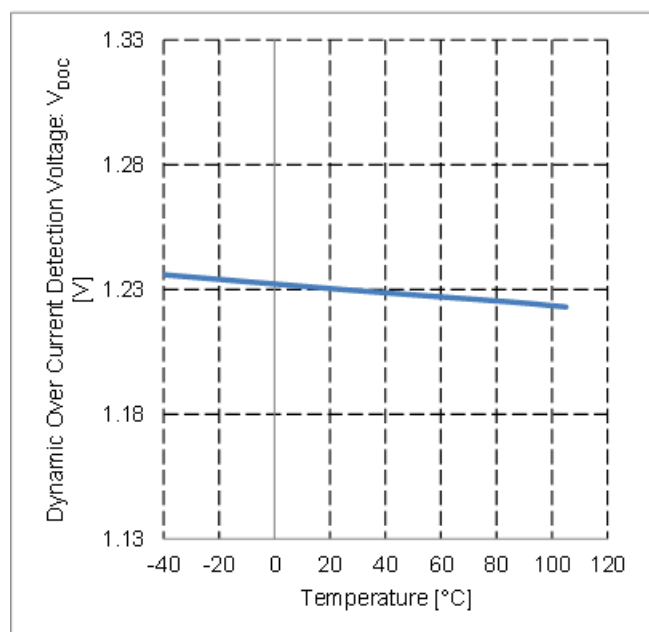
Figure 38. Dynamic Over Current Detection Voltage vs Temperature
