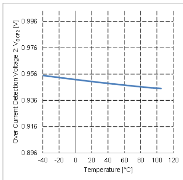
Figure 37. Over Current Detection Voltage 2 vs Temperature
