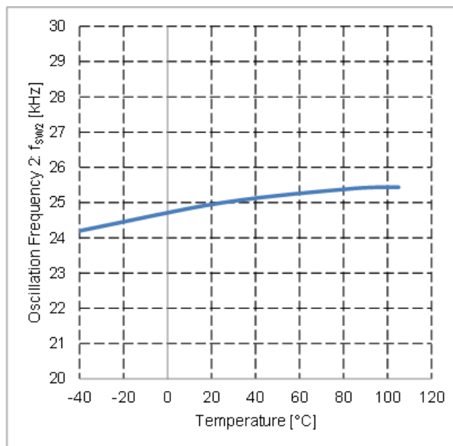
Figure 25. Oscillation Frequency 2 vs Temperature
