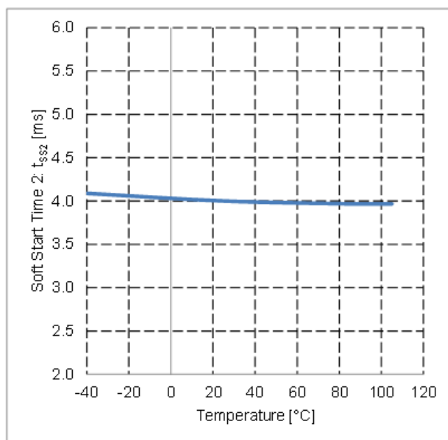
Figure 27. Soft Start Time 2 vs Temperature
