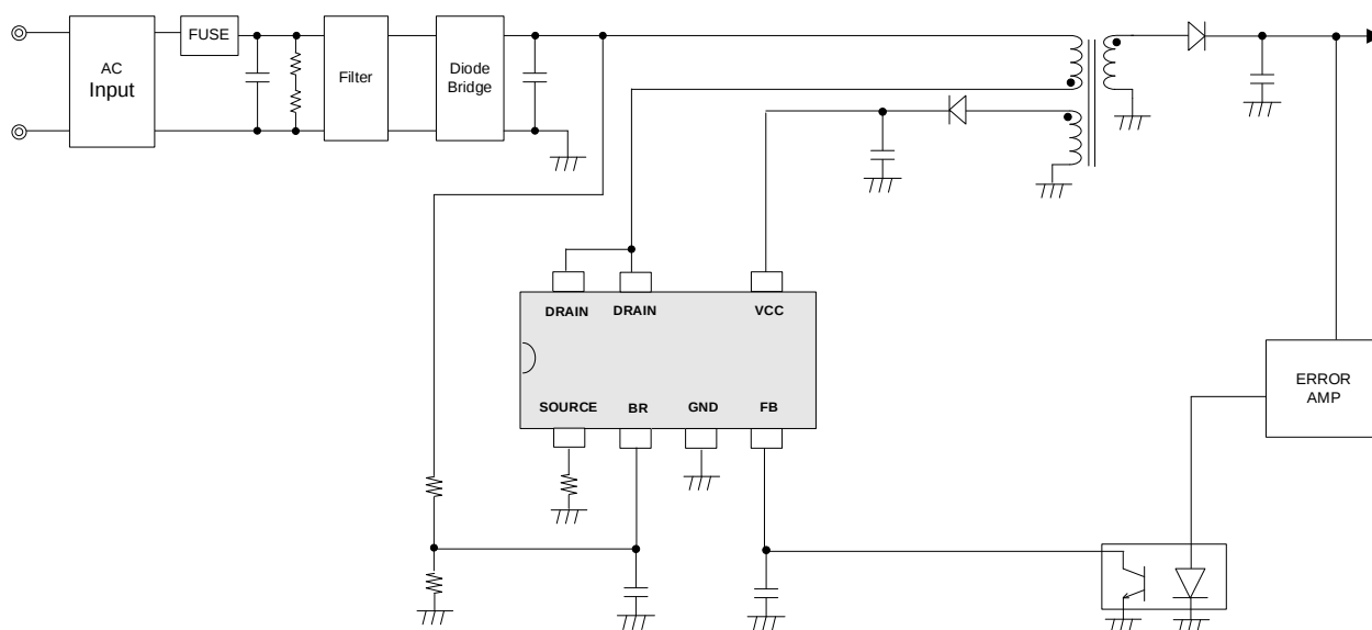
Figure 14. Flyback Application Diagram
