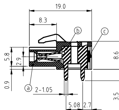
SECTION P-P
