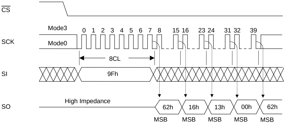
Figure 16-b. Silicon ID Read 2
