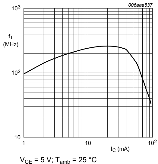
Fig. 8. TR1 (NPN): Transition frequency as a function of collector current; typical values
