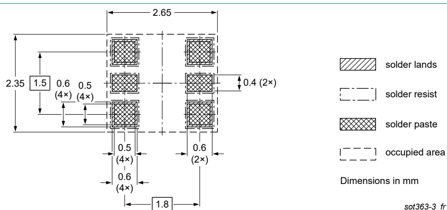
Fig. 20. Reflow soldering footprint for TSSOP6 (SOT363-3)
