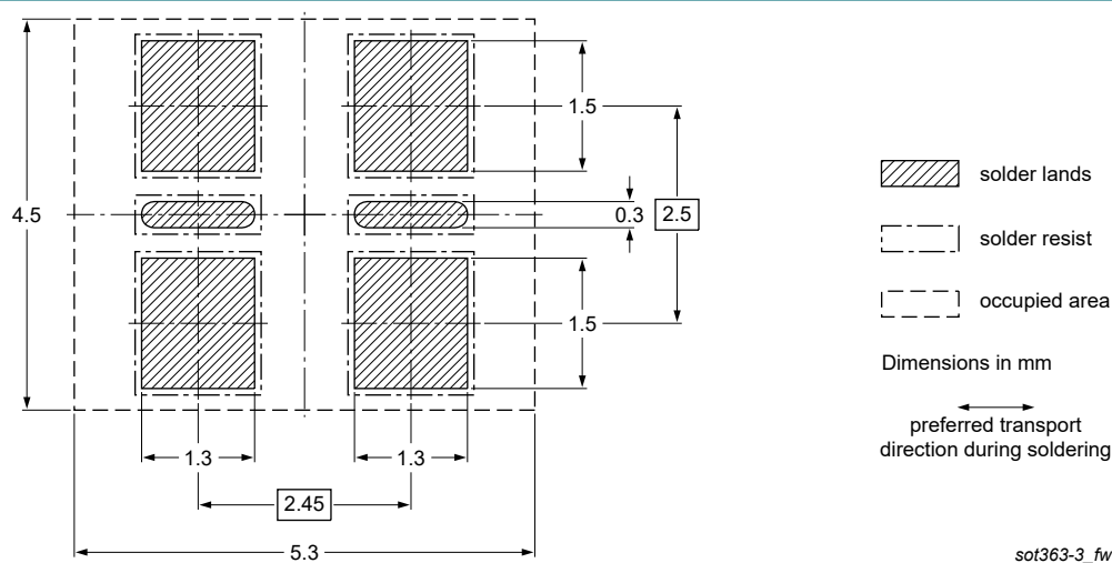
Fig. 21. Wave soldering footprint for TSSOP6 (SOT363-3)
