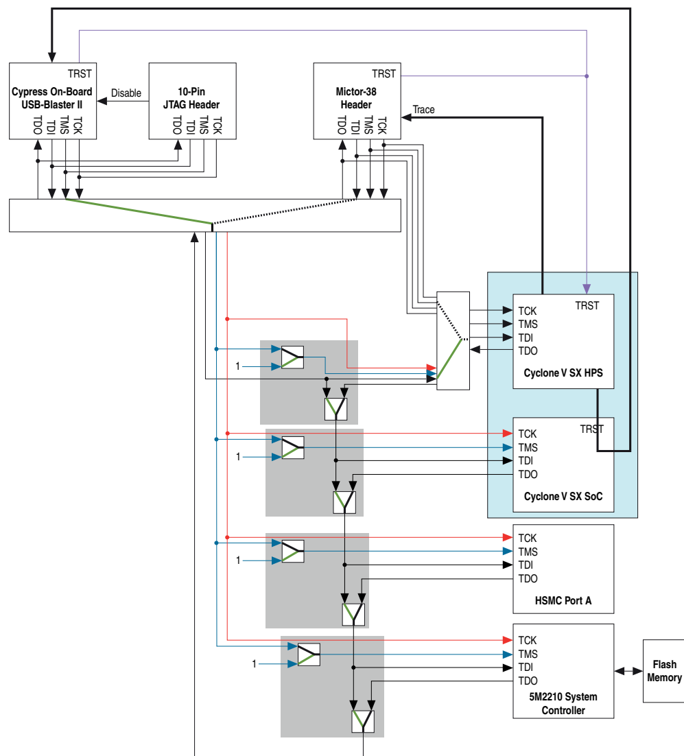
Figure 2-3. JTAG Chain
