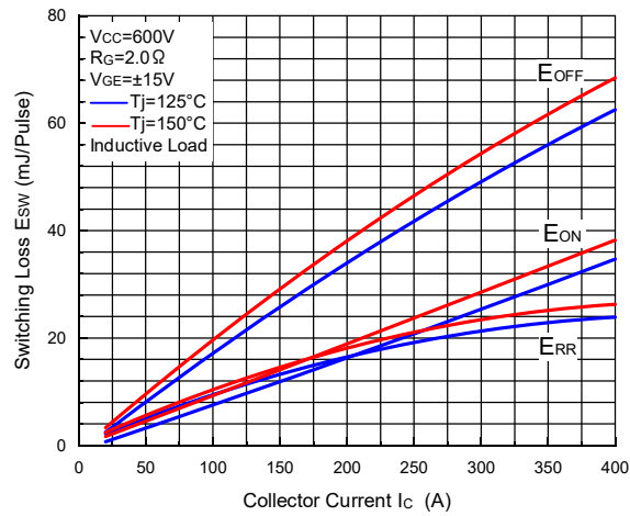
Fig.7- Collector Current vs. Switching Loss
