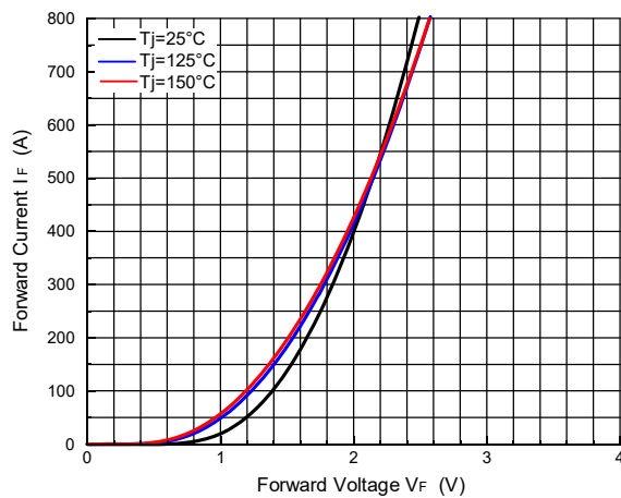
Fig.9- Forward Characteristics of FWD (Typical)
