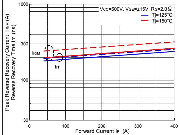
Fig.10- FWD Reverse Recovery Characteristics (Typical)
