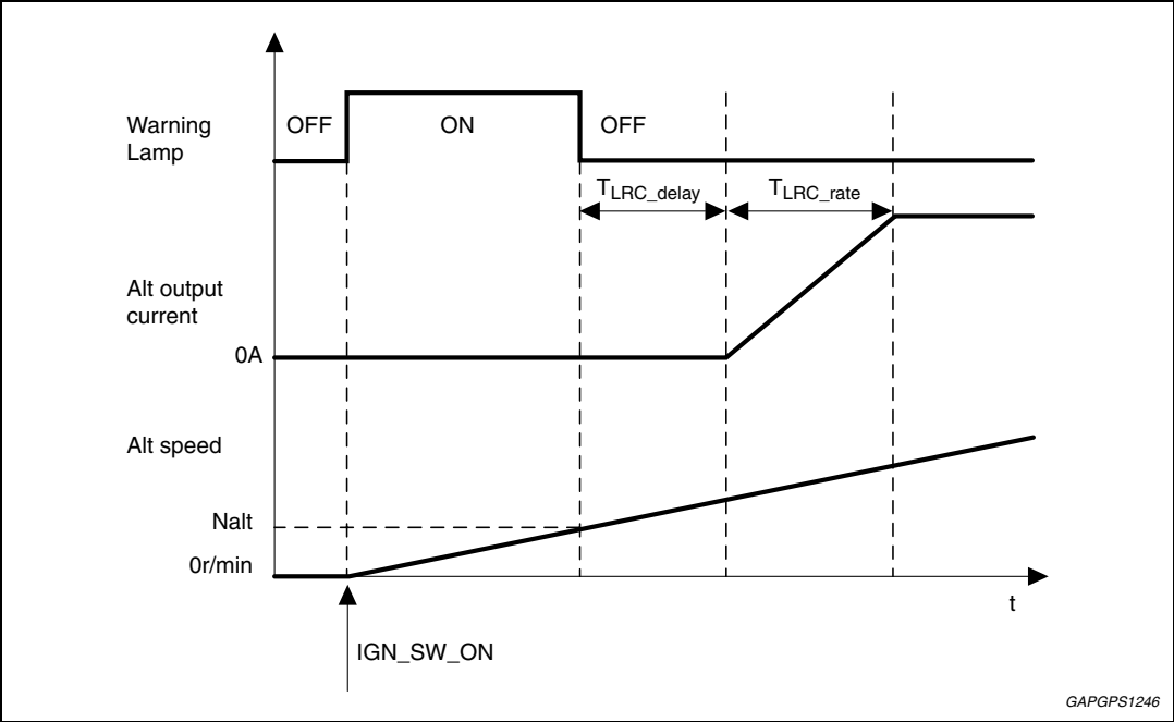
Figure 4. LRC function
