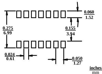
PAD LAYOUT
