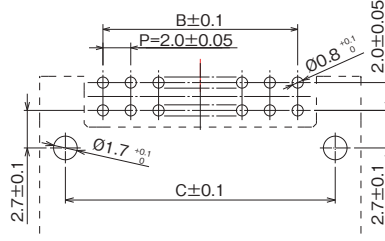
Above drawing is guide-boss type.
