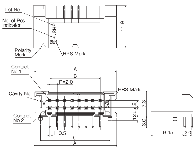
Above drawing is guide-boss type.
