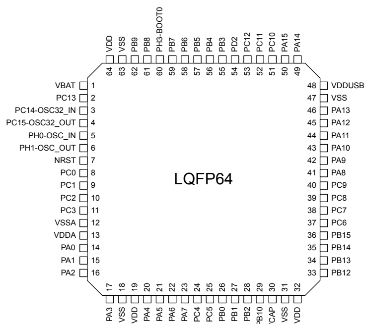
Figure 11. LQFP64 pinout
