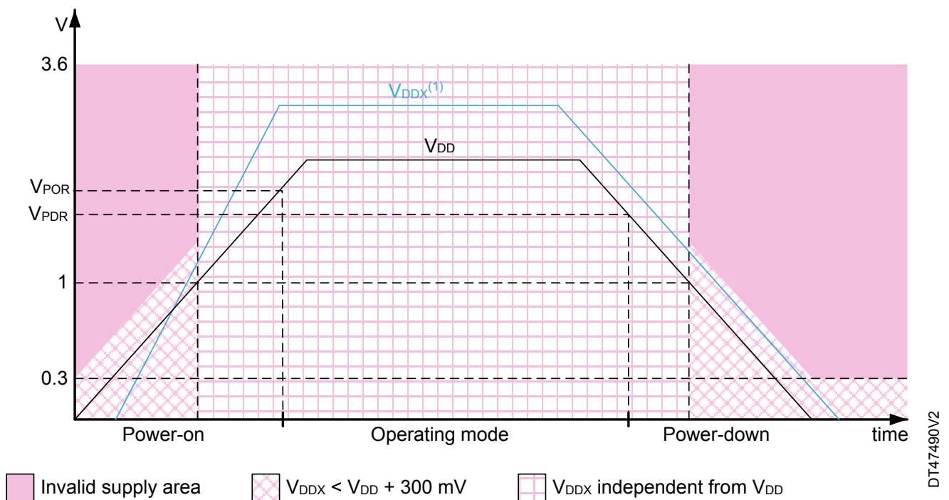
Figure 4. Power-up/down sequence
