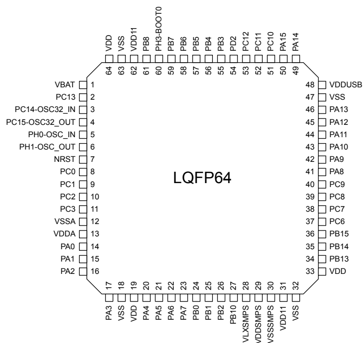
Figure 11. LQFP64 pinout
