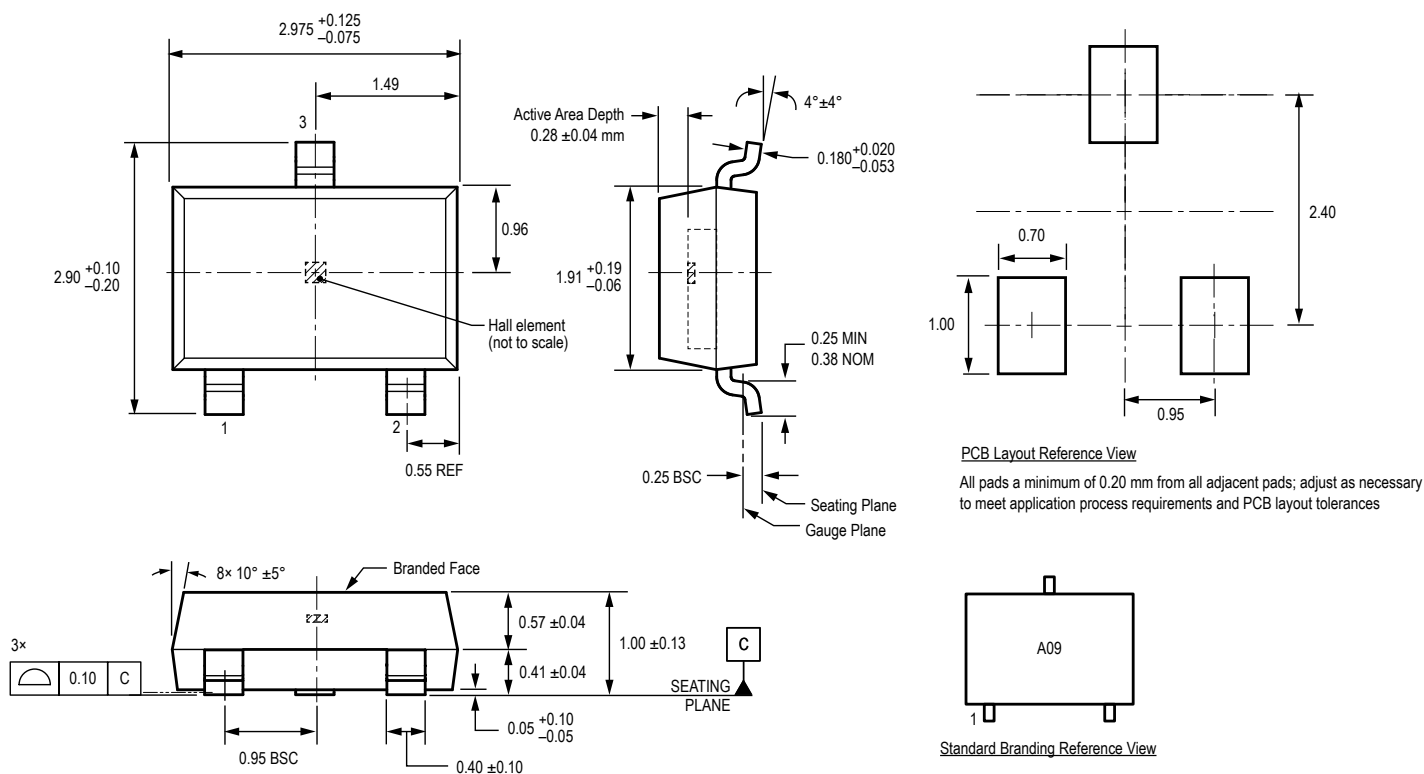
Figure 9: Package LH, 3-Pin SMD (SOT23W), APS11700
