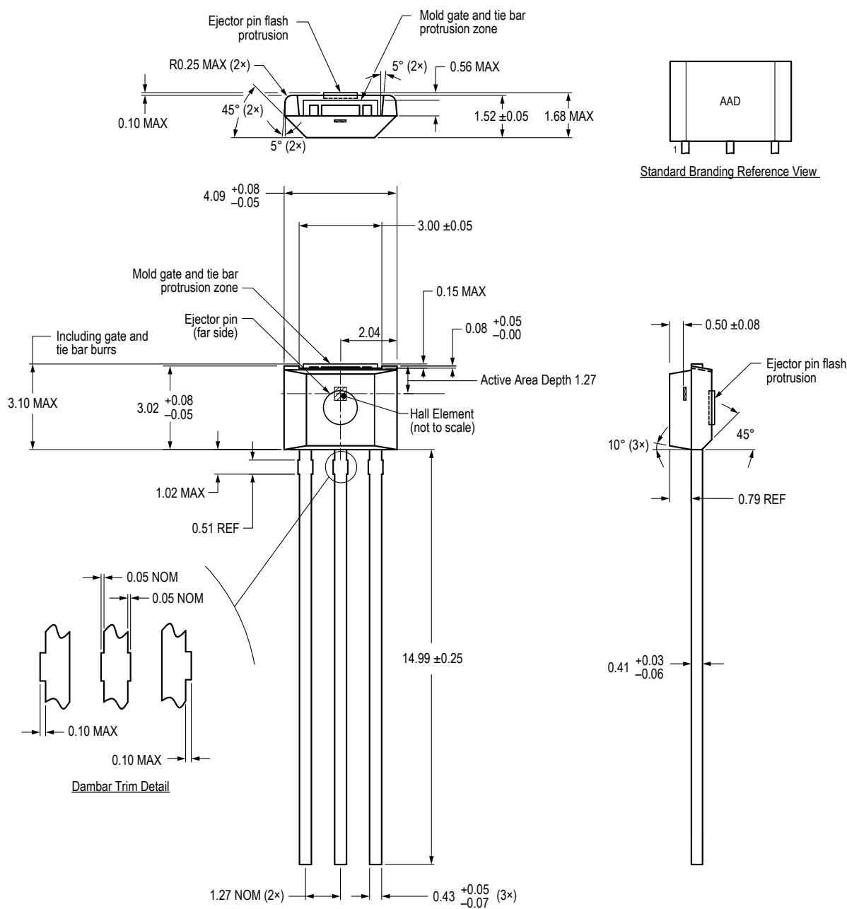
Figure 12: Package UA, 3-Pin SIP, APS11760
