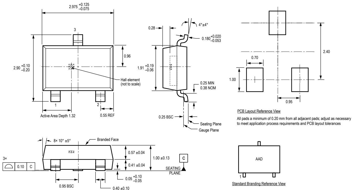
Figure 11: Package LH, 3-Pin SMD (SOT23W), APS11760
