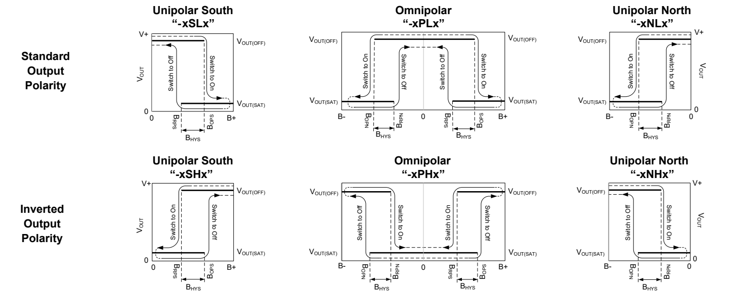
Figure 3: Hall Switch Output State vs. Magnetic Field
