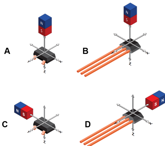
Figure 6: Magnetic Sensing Orientations APS11700 LH (Panel A), APS11700 UA (Panel B), APS11760 LH (Panel C), and APS11760 UA (Panel D)
