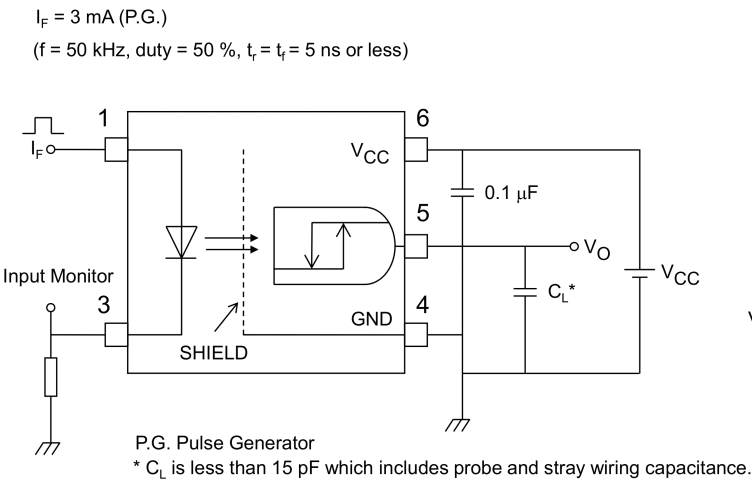
Fig. 12.1.8 Switching Time Test Circuit and Waveform
