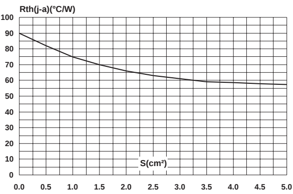
Fig. 10: Thermal resistance junction to ambient versus copper surface under each lead (epoxy FR4, e = 35\mu\text{m} ).
