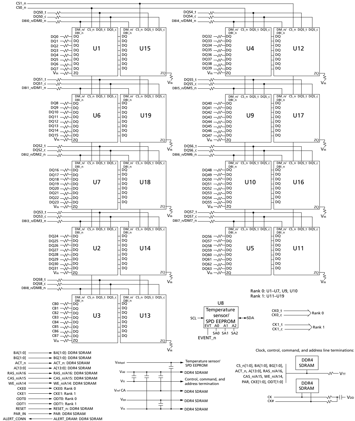
Figure 3: Functional Block Diagram (R/C-F, PCB 1742)
