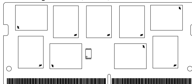
Figure 2: 260-Pin SODIMM (MO-310 R/C H)
