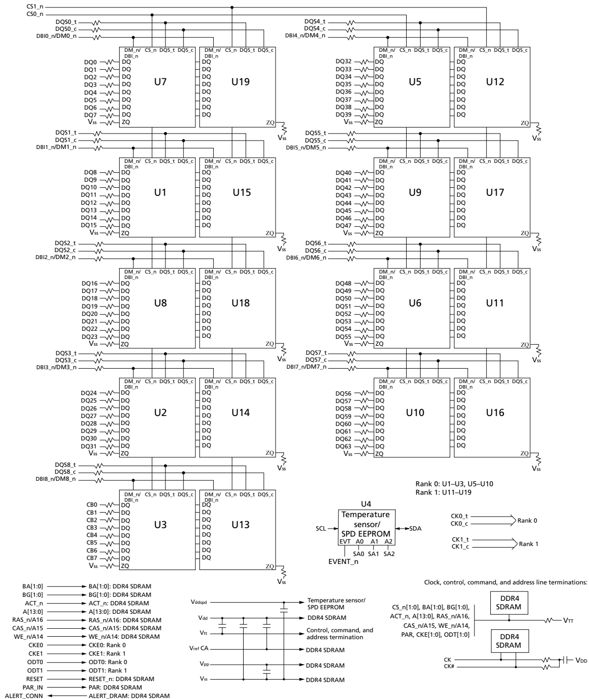
Figure 4: Functional Block Diagram (R/C-H, PCB 1813)
