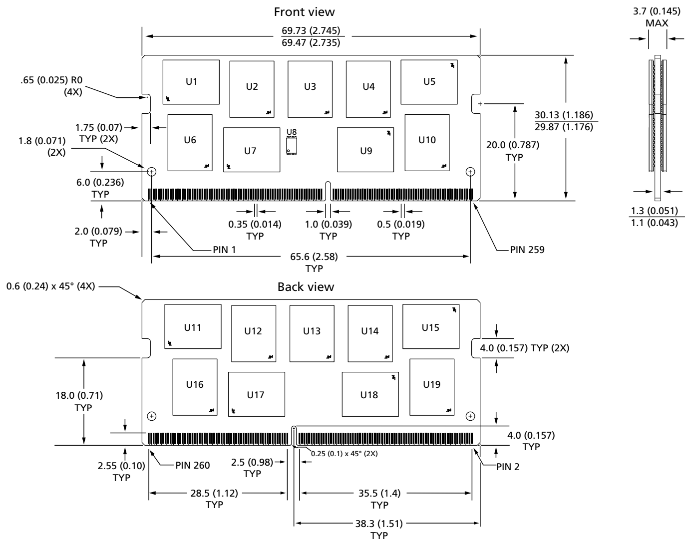
Figure 5: 260-Pin DDR4 SODIMM (R/C-F)
