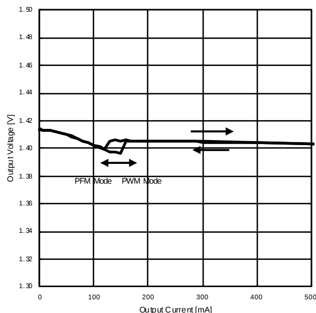
Figure 28. Output Voltage vs Output Current (SWREG4 Load Regulation)
