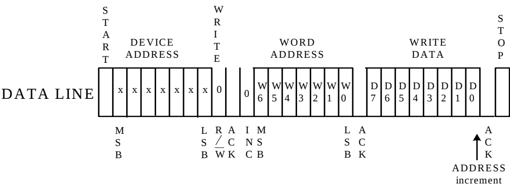
Figure 14. Write Operation
