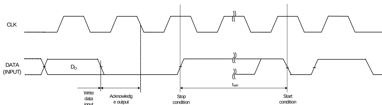
Figure. 9 Bus Timing 2
