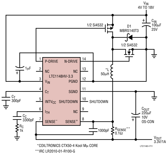
Figure 11. High Efficiency 5V to 3.3V/1A Converter with Extended Input Voltage Range
