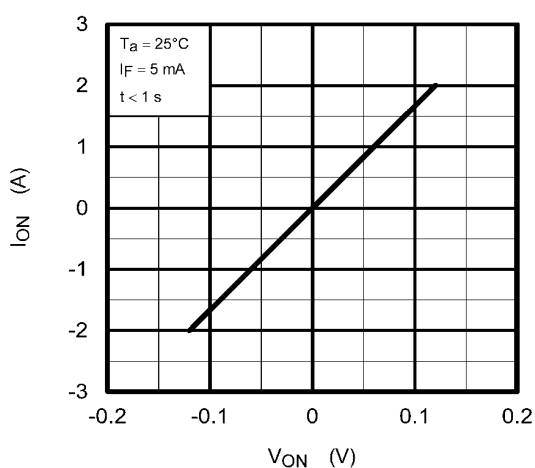
Fig. 16.4 I ON - V ON
