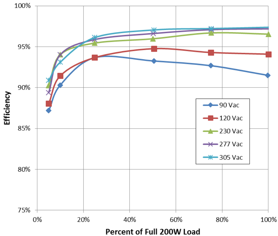
Figure 8. Efficiency
