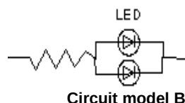
(B) The brightness of each LED might appear different due to the differences in the I-V characteristics of those LEDs.
