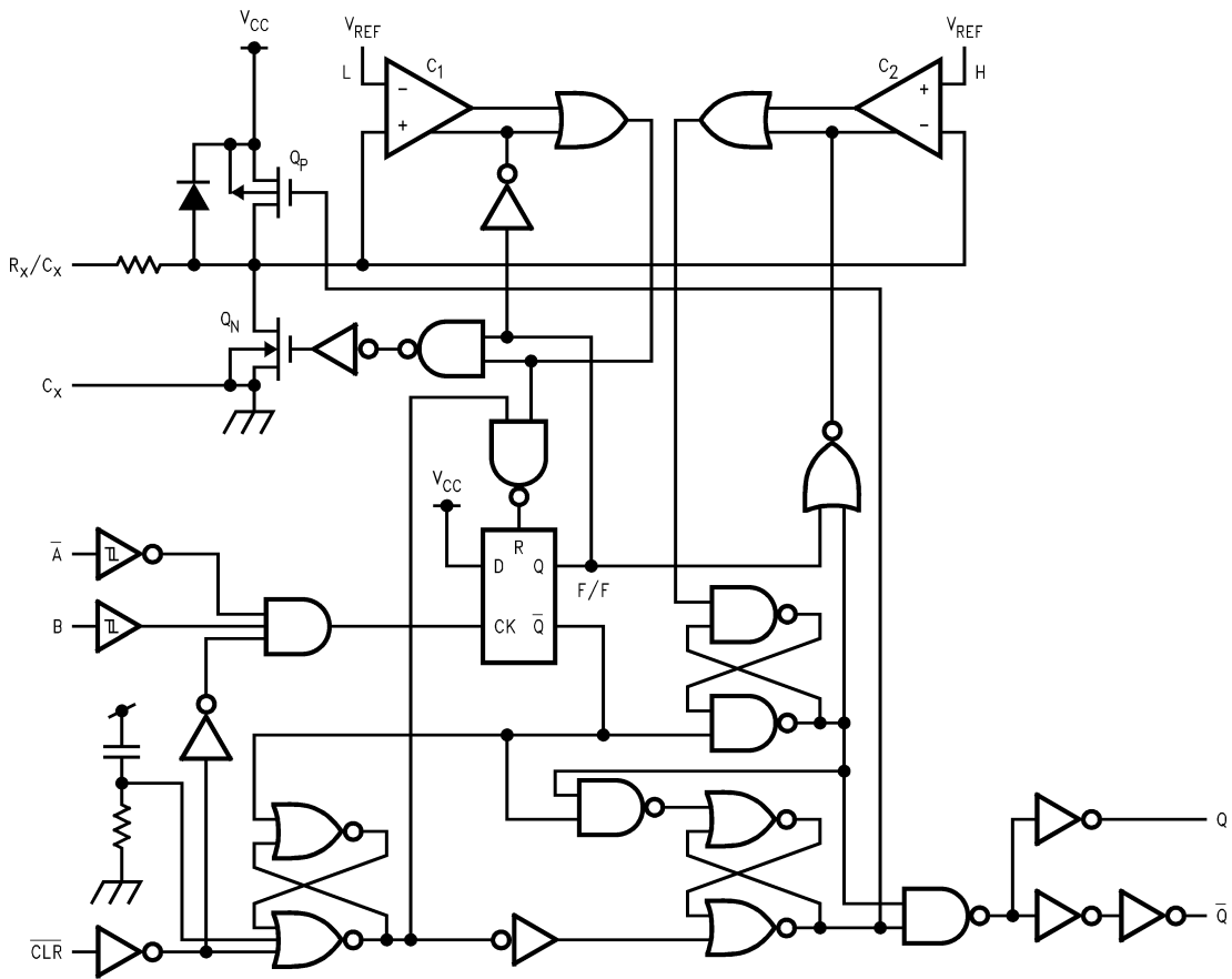
Figure 4. System Diagram
