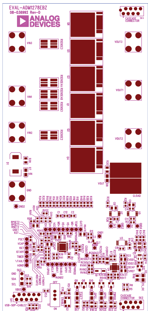
Figure 19. Assembly Top
