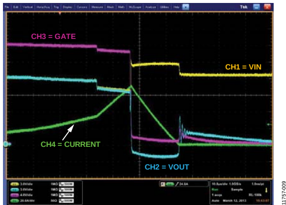
Figure 10. Output Short Circuit (Zoom-In)
