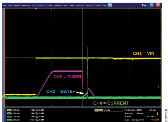
Figure 11. Power Up into Short
