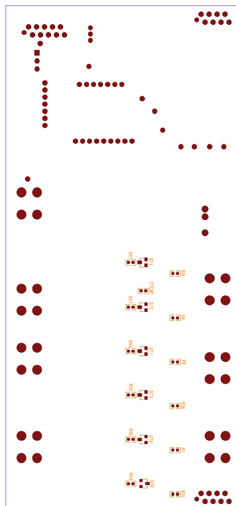
Figure 20. Assembly Bottom
