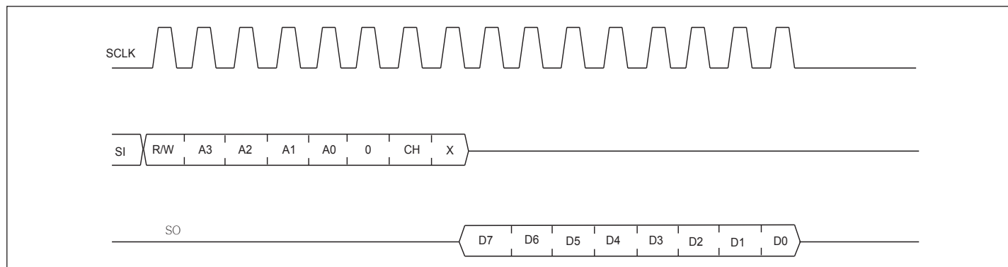
Figure 14. SPI Read
