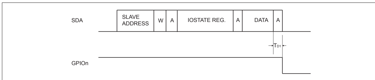
Figure 20. Write to Output
