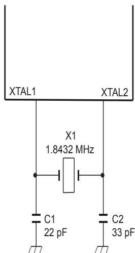
Figure 8. Crystal Oscillator Circuit Reference
