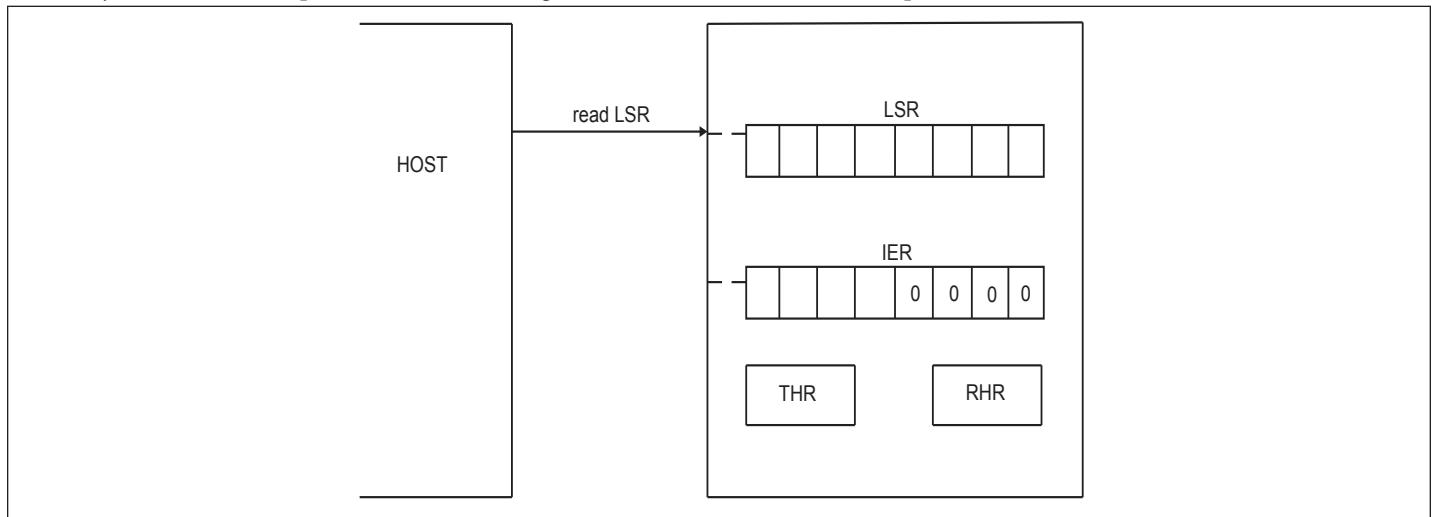
Figure 6. FIFO Polled Mode Operation
