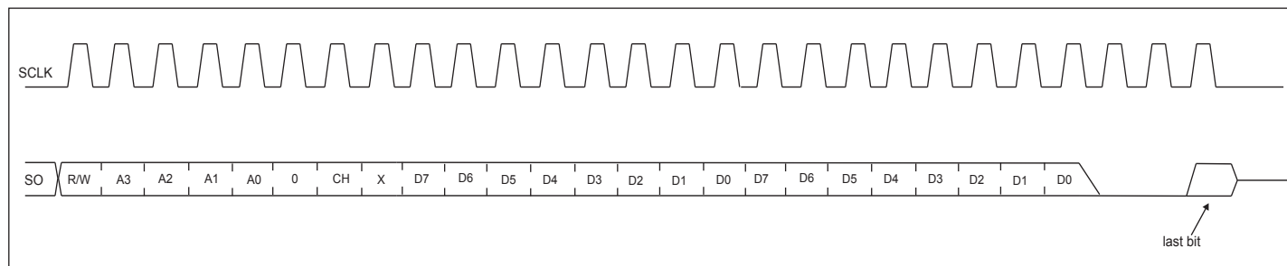
Figure 15. SPI FIFO Write
