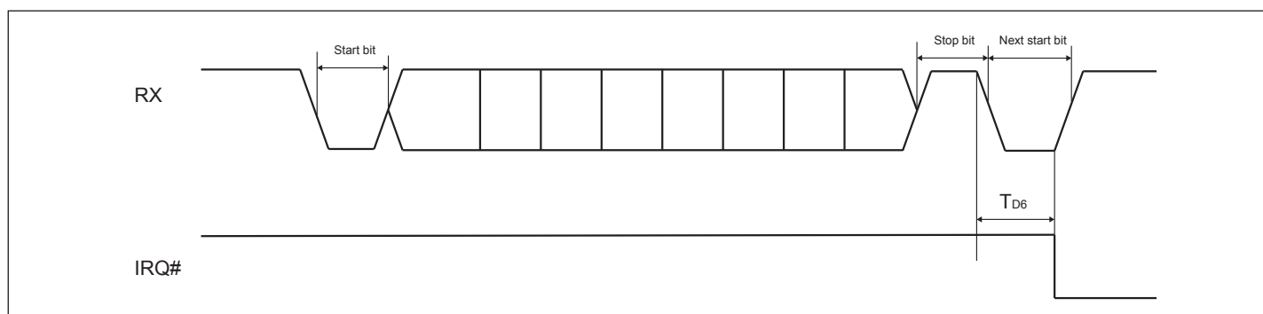
Figure 23. Receive Interrupt
