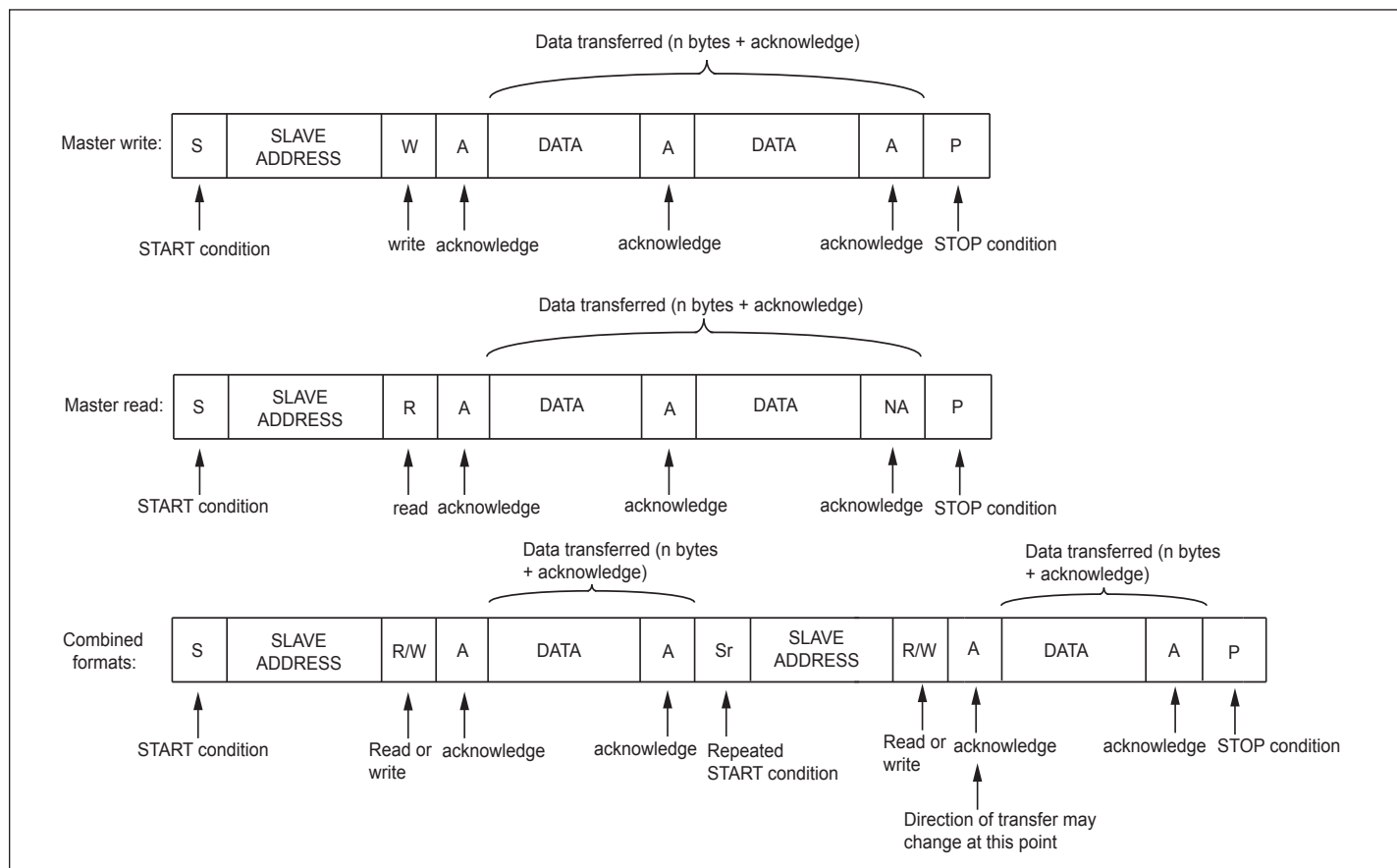
Figure 12. I²C Data Formats
