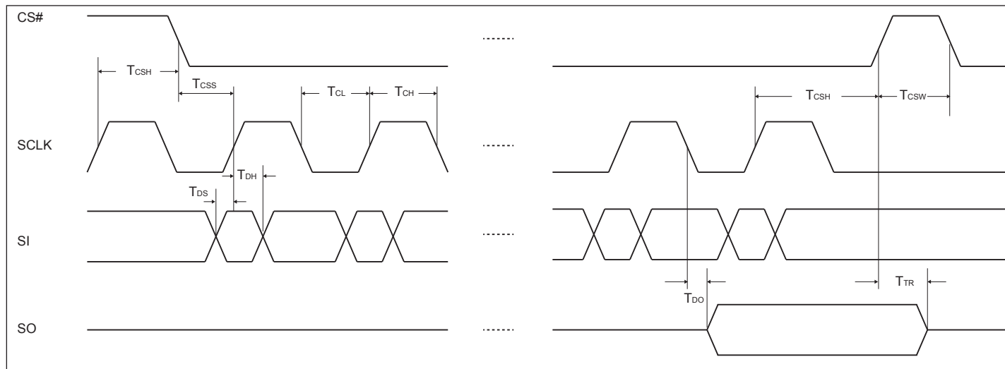
Figure 26. SPI-Bus Timing
