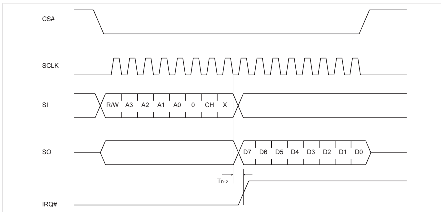
Figure 30. Read MSR to Clear Modem INT
