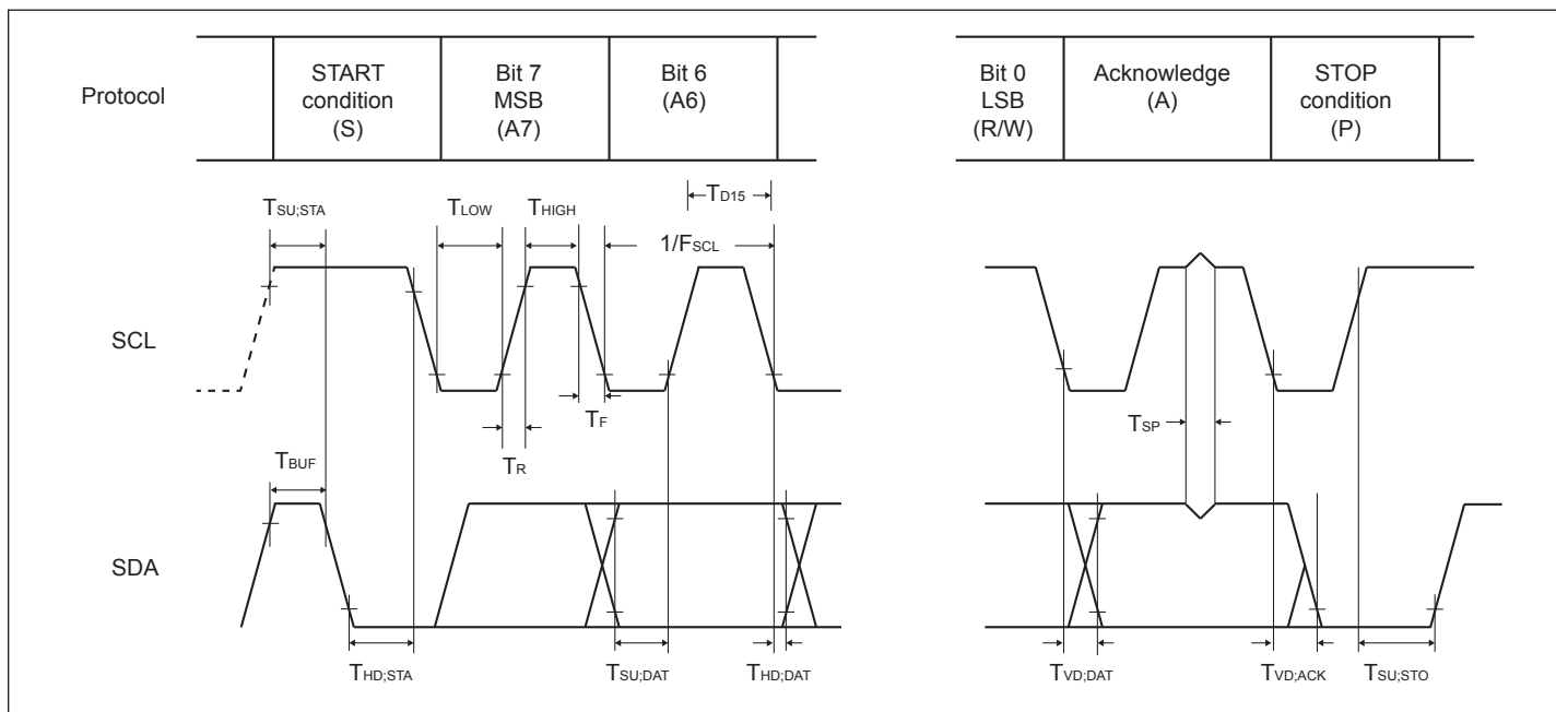
Figure 19. I²C-Bus Timing Diagram
