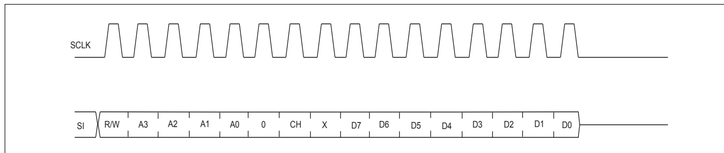
Figure 13. SPI Write
