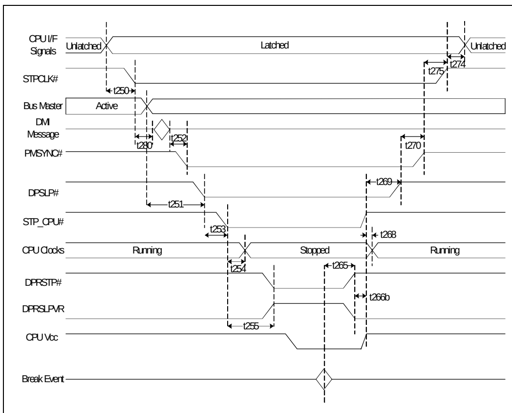
Figure 8-23. Sleep control signal relationship - Host boots and Management Engine off
