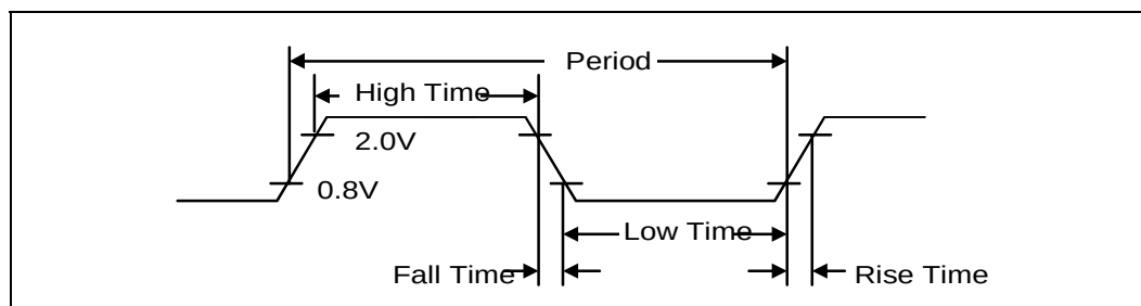
Figure 8-1. Clock Timing
