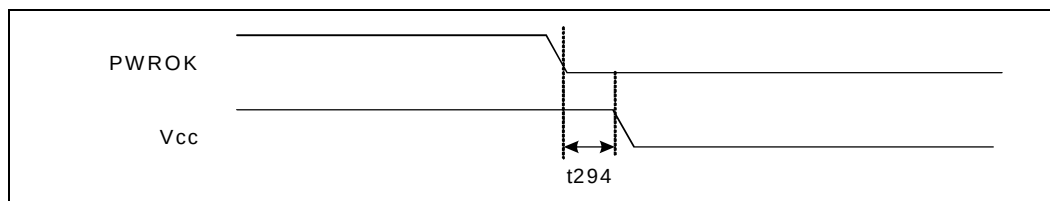
Figure 8-28. S0 to G3 Timings (Mobile Only)
