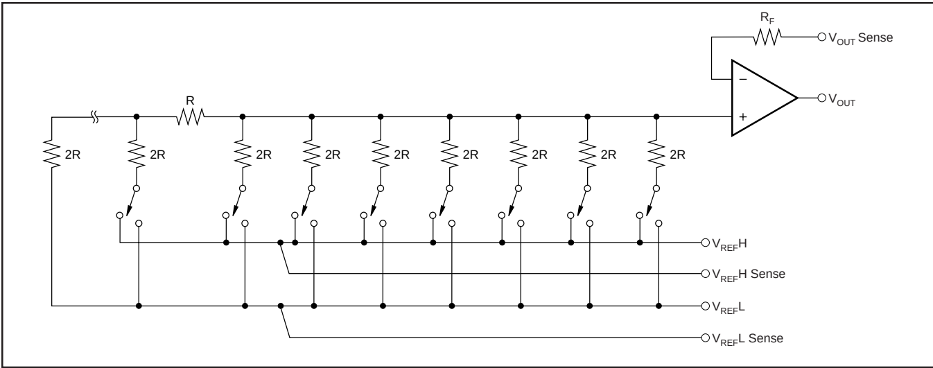
FIGURE 1. DAC7744 Architecture.
