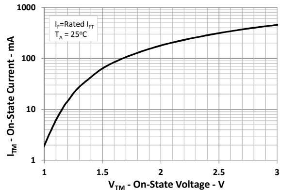
Fig.8 Normalized I_{TM} vs. V_{TM}
