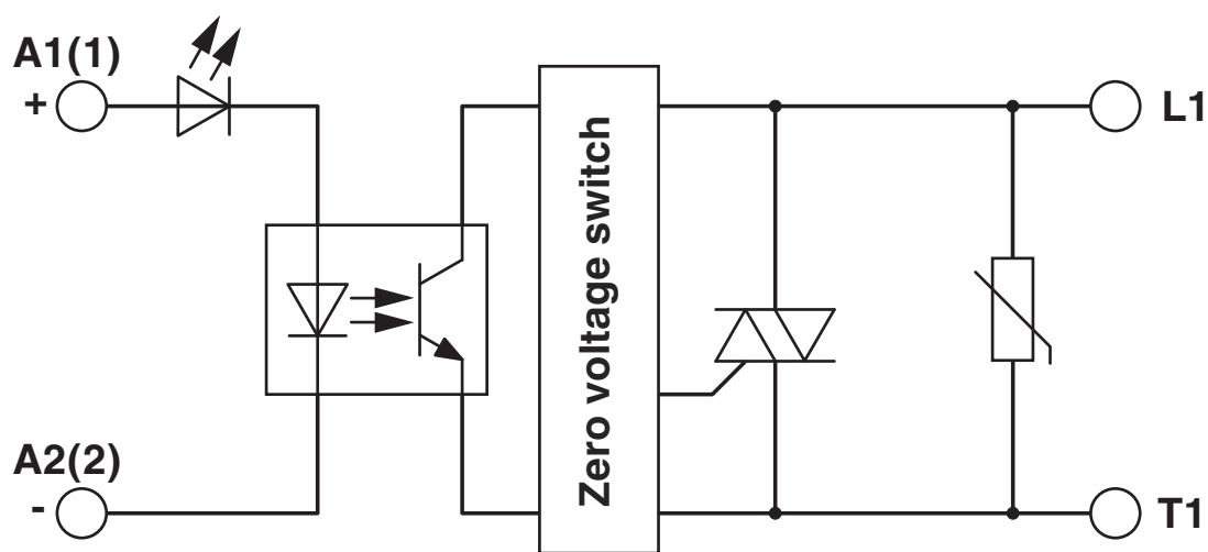
Block diagram
