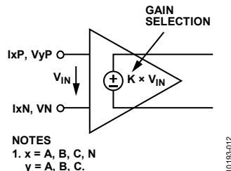
Figure 37. Maximum Input Level, Voltage Channels, Gain = 1
