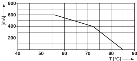
Derating curve at 30 V AC
