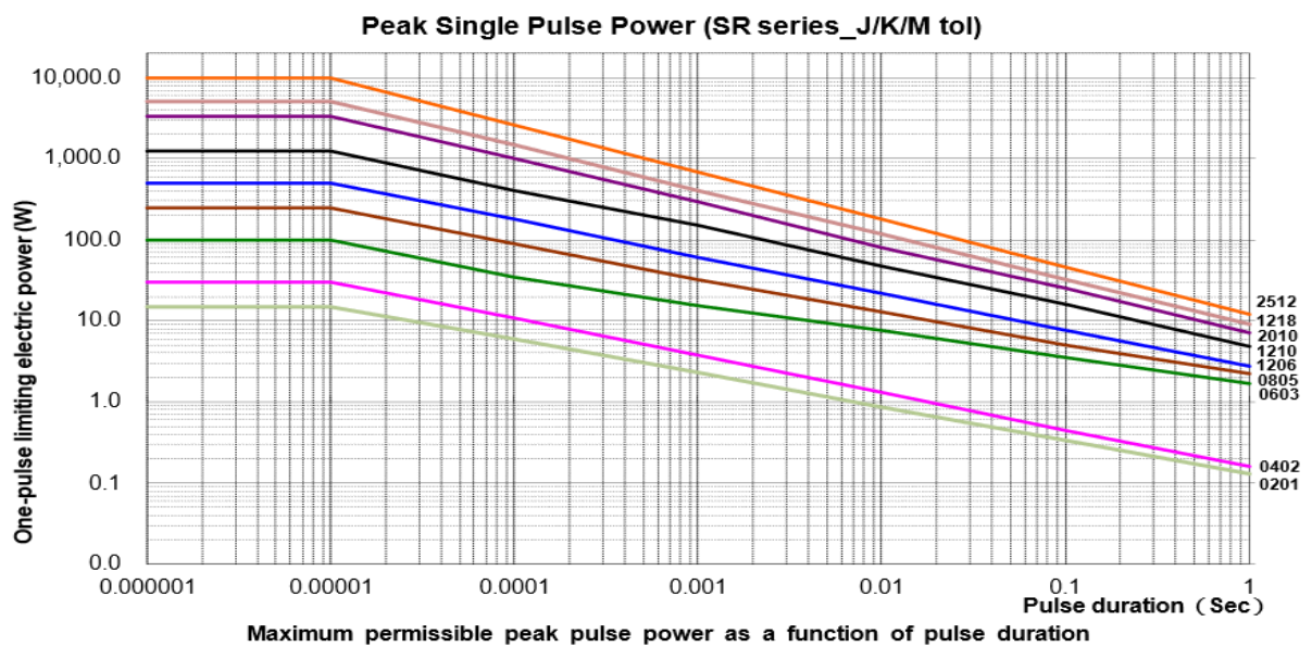
Fig. 7-2 Pulse-Load behavior
