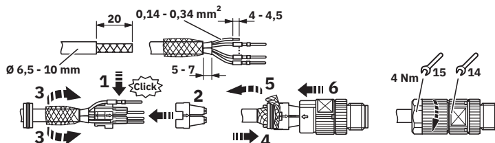
Functional drawing
