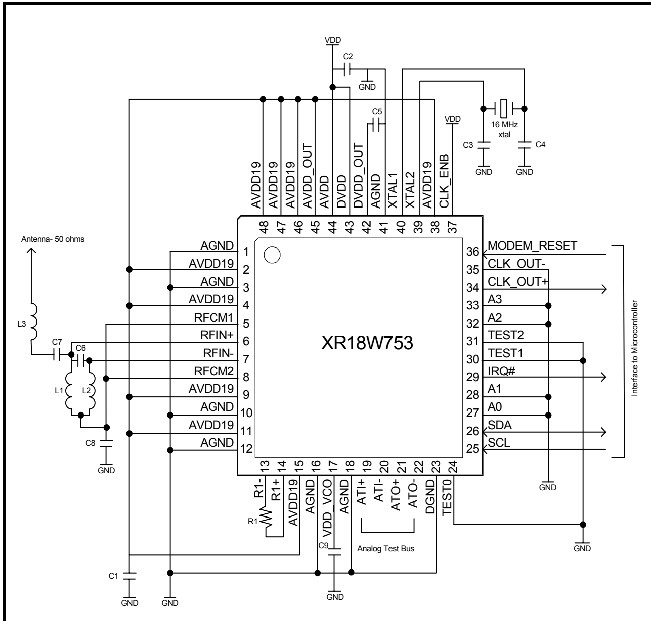
FIGURE 4. APPLICATION DIAGRAM
