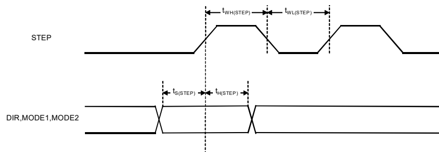
Figure 3. Timing Chart
