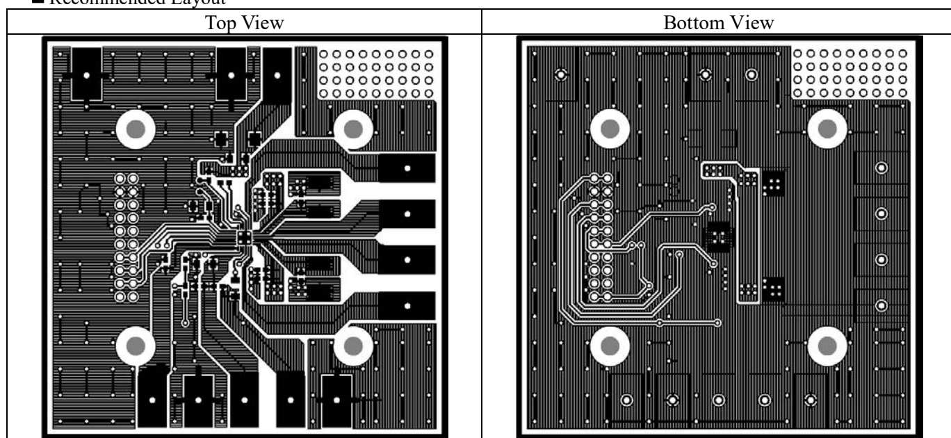
Figure 15. Recommended Layout Pattern
