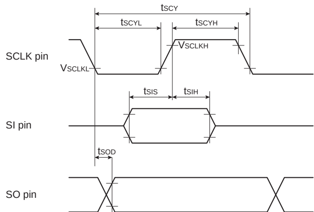
Figure 19-17 AC Characteristics
