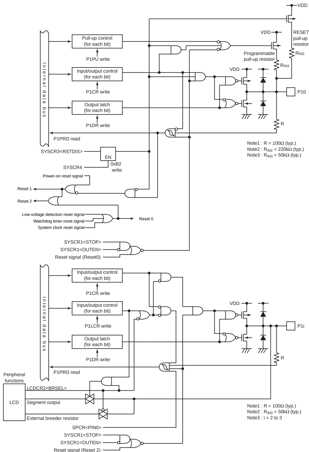
Figure 8-4 Port P1
