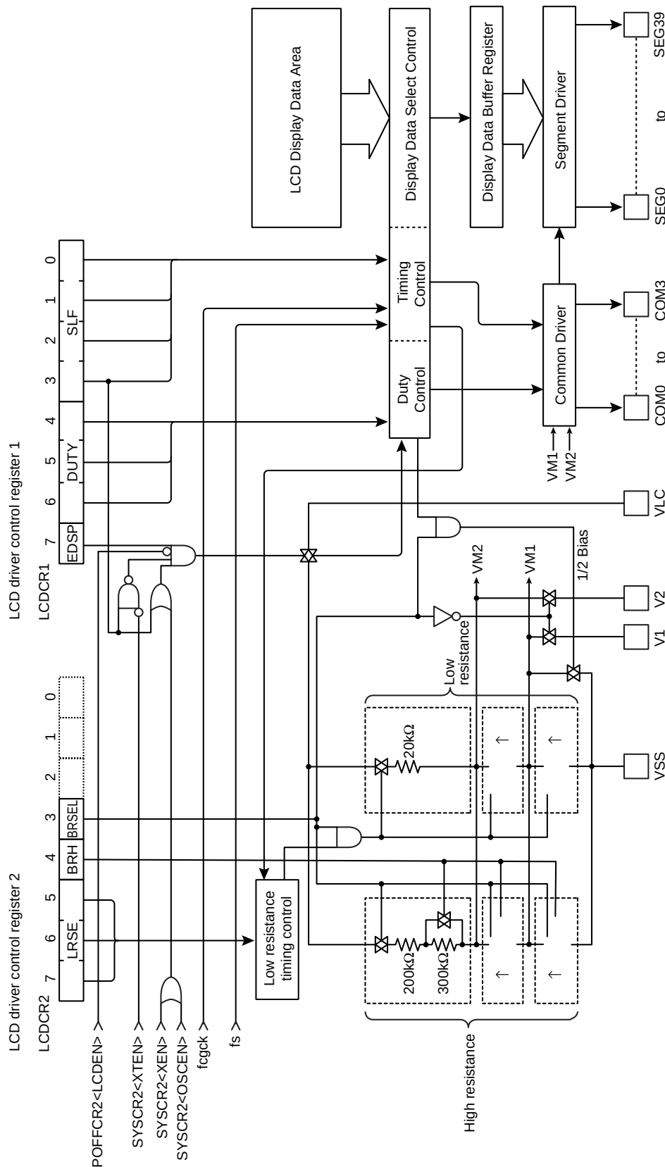
Figure 23-1 LCD Driver
