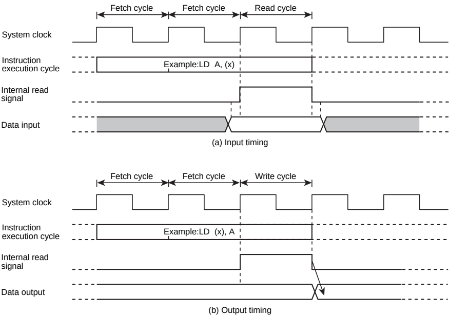
Figure 8-1 Input/Output Timing(Example)
