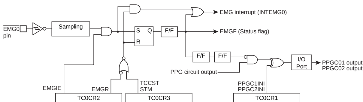
Figure 15-22 \overline{\text{EMG0}} Pin
