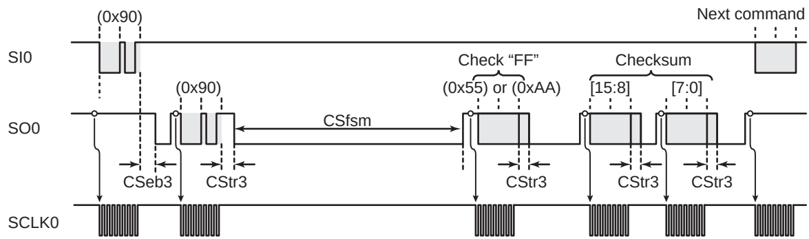
Figure 26-22 Flash Memory SUM Output Command
