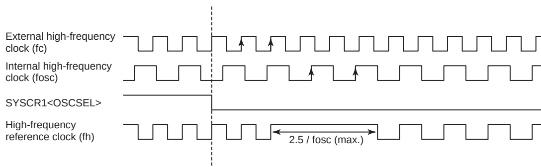
Figure 2-6 Switching the High-Frequency Reference Clock (fh) (fc to fosc)
