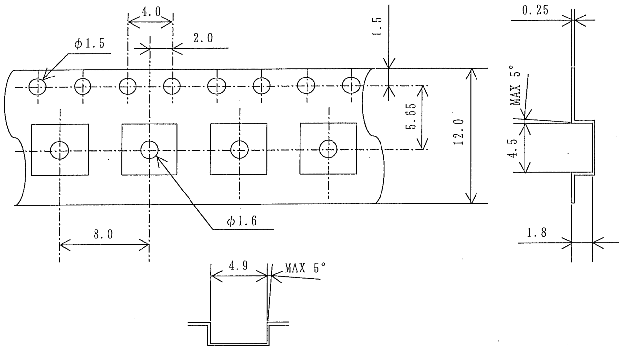
Fig. A Tape structure and Dimensions
