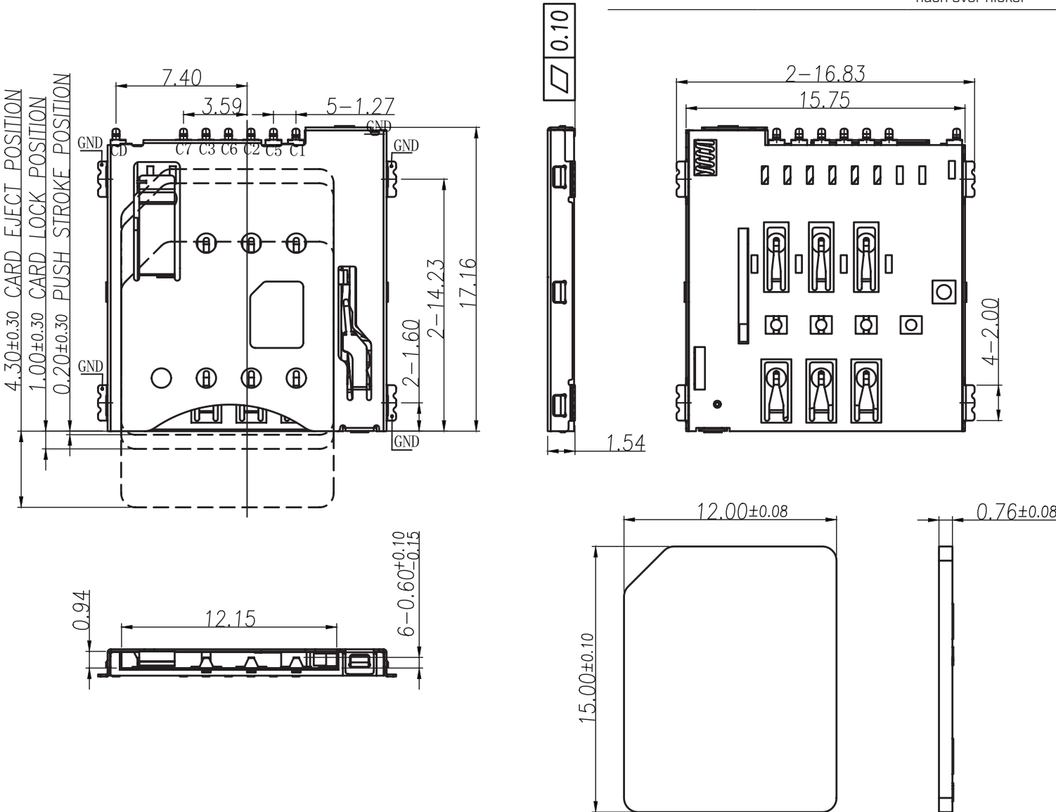
MICRO SIM
