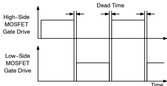
Figure 15. MOSFETs Gate Drive Signal
