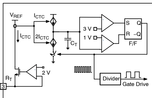
Figure 16. Current-Controlled Oscillator
