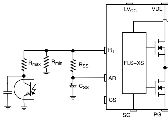
Figure 18. Frequency Control Circuit
