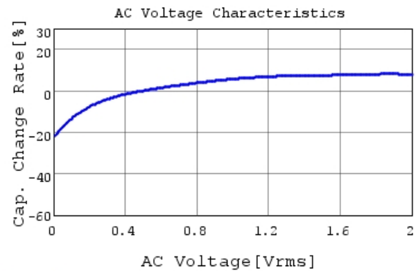
GRT21BR61C226ME13 C-AC Voltage capchange, D
