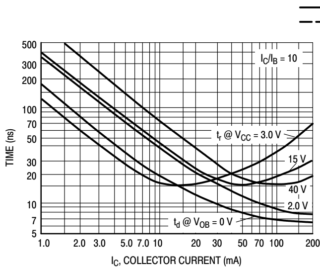
Figure 4. Turn - On Time
