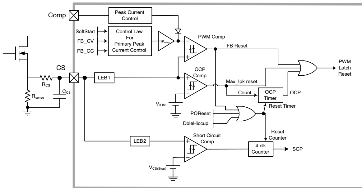
Figure 38. Current Setpoint
