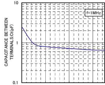
VR-Ct CHARACTERISTICS
