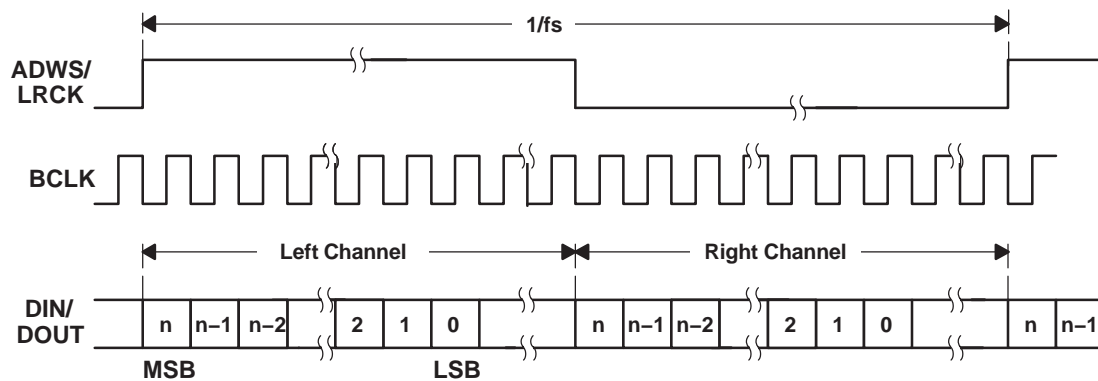
Figure 15. Timing Diagram for Left-Justified Mode
