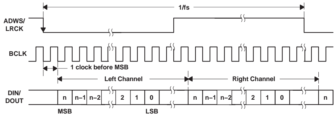
Figure 16. Timing Diagram for I 2 S Mode
