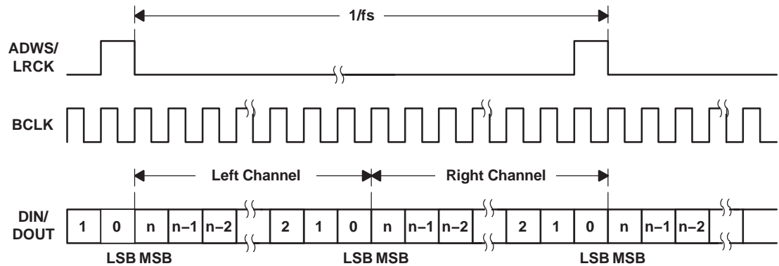
Figure 17. Timing Diagram for DSP Mode
