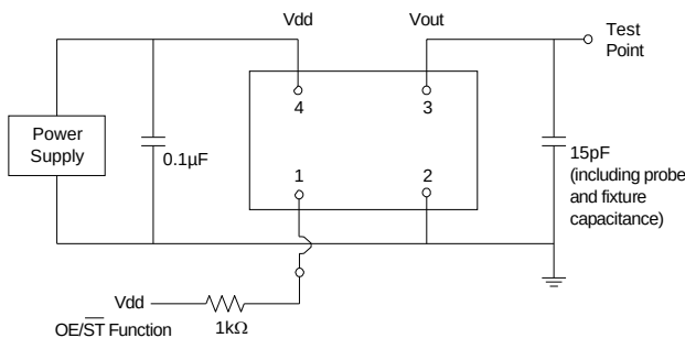
Figure 2. Test Circuit
