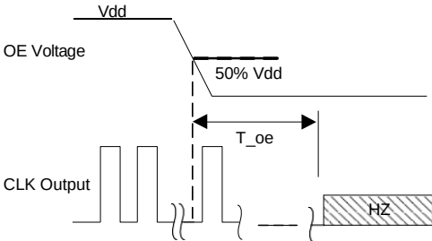
Figure 7. OE Disable Timing (OE Mode Only)
