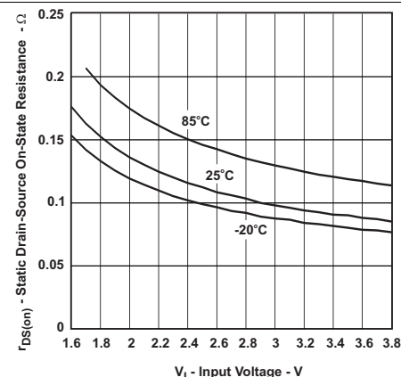
Figure 4. PMOS R_{DS(on)} vs Input Voltage
