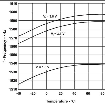
Figure 3. Frequency vs Temperature
