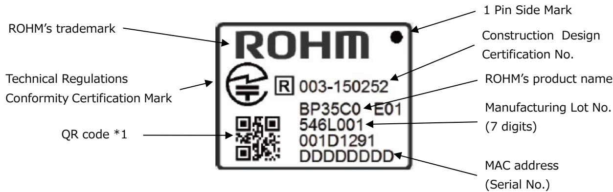
Fig. 4. Marking Specification
